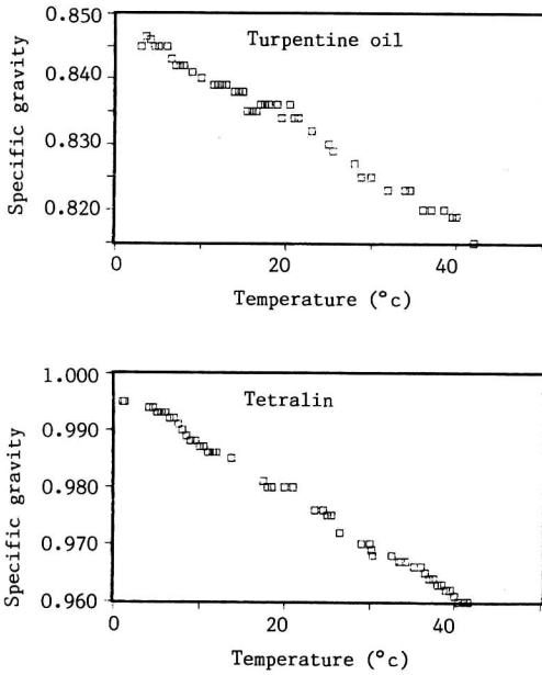
Fig.2 Variation of specific gravity of solvents with temperature.
