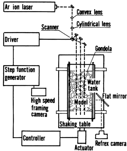
Fig.13 Apparatus for dynamic failure test.
