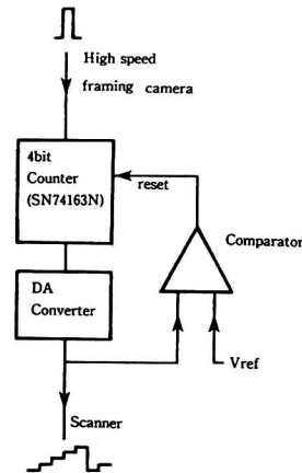
Fig.6 Step function generator.
