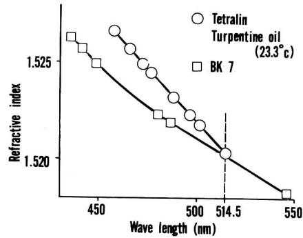
Fig.5 Variation of refractive index with wave length.
