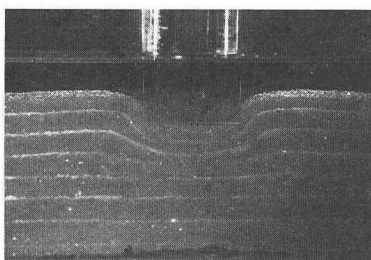
Fig.11,d Settlement, s = 15 mm.
