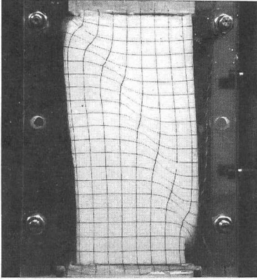
Fig.12 Failure pattern of the glass particles in PSC test, at \epsilon_a = 12\% , \sigma_c = 0.05 \text{ kgf/cm}^2 and c = 0.840 .
