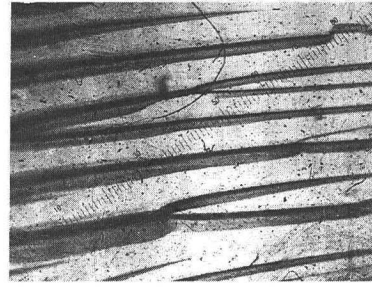
Fig.4 Hackle Marks on a surface of BK-7 (Magnification:100).
