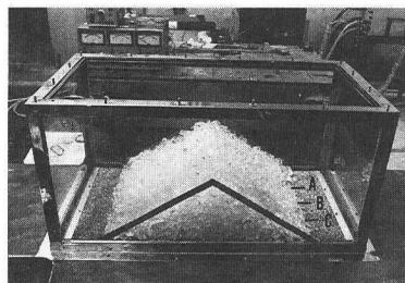
Fig. 8,a Embankment model.
