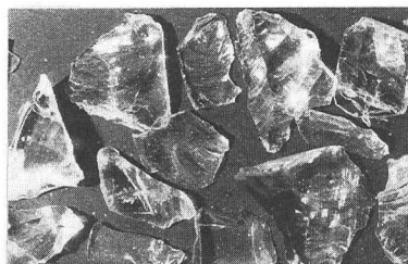
Fig.10 Micrograph of the glass grains at magnification of 10 times.
