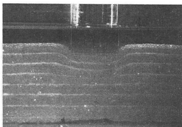
Fig.11,c Settlement, s = 10 mm.
