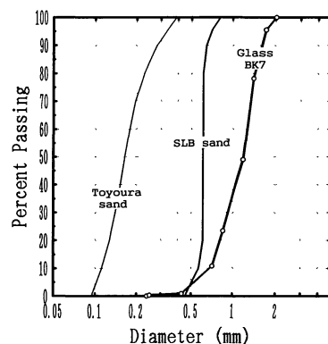
Fig.9 Particle size distribution curves.
