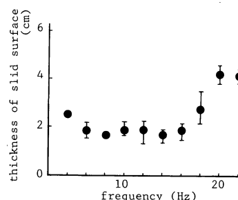
Fig.17 Variation of thickness of slid surface with frequency.
