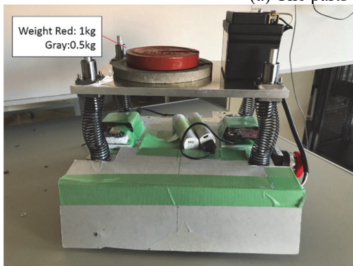
(b) The vehicle model with the weights
