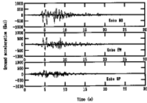
Fig.3 Great Hanshin-Awaji Earthquake accelerogram used in the analysis
