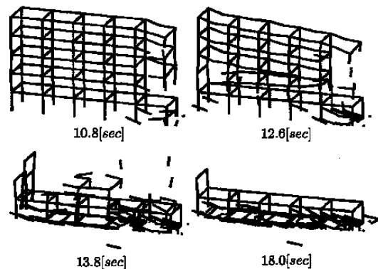
Fig.4 Seismic damage analysis of reinforced concrete building using ASI technique
